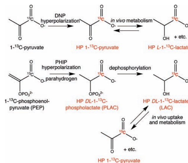
Figure 1. Molecular diagrams of PHIP and DNP hyperpolarization of 1\text{-}^{13}\text{C} -pyruvate and 1\text{-}^{13}\text{C} -phospholactate (PLAC) and their metabolism for application as metabolic hyperpolarized (HP) agents.
