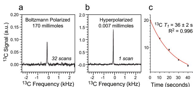
Figure 3. ^{13}\text{C} NMR spectroscopy conducted at 0.0475 T. (a) ^{13}\text{C} reference spectrum of 170 mmol (14 g in 50 mL \text{D}_2\text{O} ) of sodium 1\text{-}^{13}\text{C} -acetate, Boltzmann polarization at 308 K, 32 averages. (b) ^{13}\text{C} spectrum of 0.007 mmol, 1.5 mg in 3.6 mL \text{H}_2\text{O} at pH = 9.0, hyperpolarized potassium DL\text{-}1\text{-}^{13}\text{C} -PLAC, polarization P = 1.0\% corresponding to signal enhancement by 240,000-fold measured by comparing ^{13}\text{C} signal intensity of hyperpolarized 0.007 mmol of PLAC with that of 170 mmol of sodium 1\text{-}^{13}\text{C} -acetate at Boltzmann polarization at 0.0475 T and 308 K (in a). 9 (c) Decay of ^{13}\text{C} hyperpolarized PLAC signal measured with 30^\circ excitation pulses. The T_1 decay was simulated (red trace) as an exponential decay taking into account the effect of RF pulses on ^{13}\text{C} magnetization.
